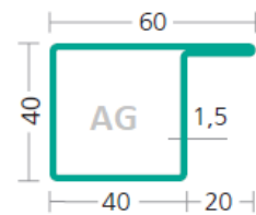
AS 4040/20 L/54101683 Edelstahl, 1.4301
